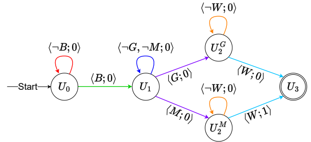
Figure 2: (a) A textual representation of the RM in Example 1 describing the Make-Coffee task. (b) A graph visualization of the textually defined RM. (c) An expansion of the RM that differentiates between mug and glass receptacles, described in Section 3.
